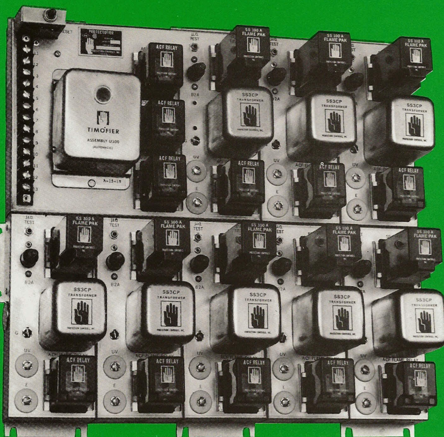
Eight Burner PROTECTOFIER
