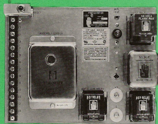
Single-Burner PROTECTOFIER
