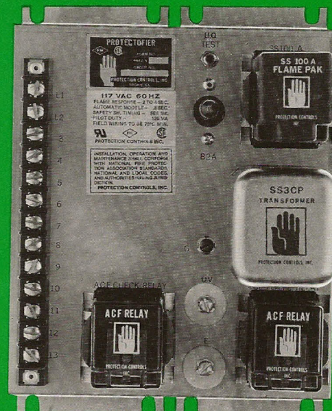
Single Burner PROTECTOFIER
