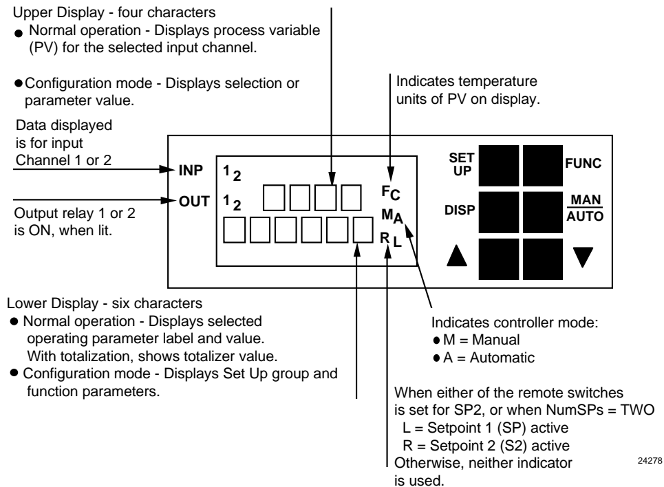
Figure 4-7 Operator Interface
