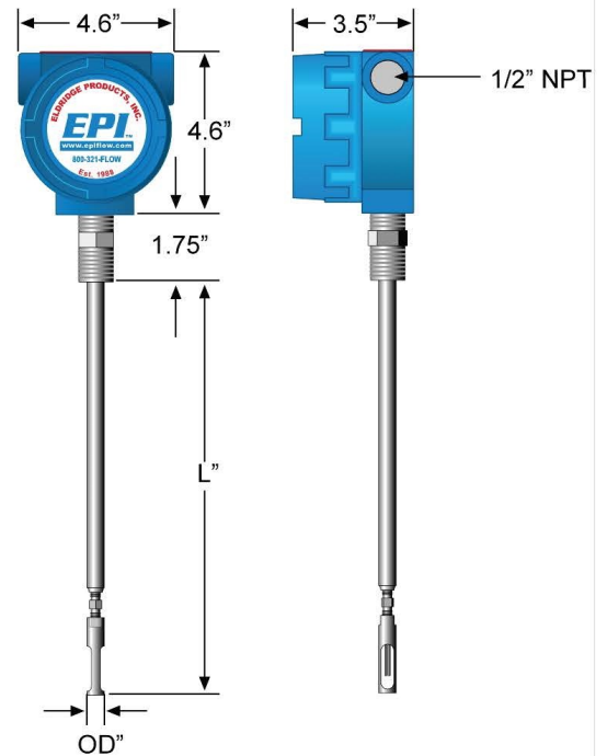
Flow Transmitter Assembly
