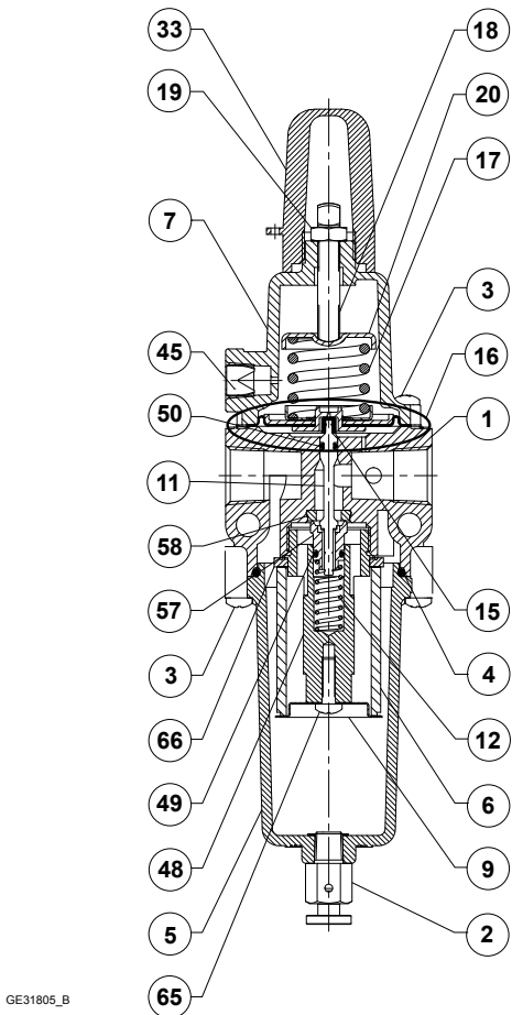
Figure 1. Types 67DFS and 67DFSR Assembly
