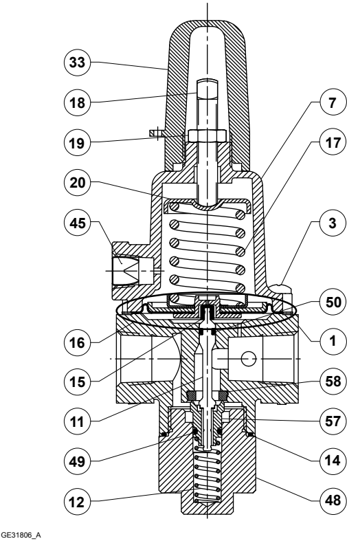
Figure 2. Types 67DS and 67DSR Assembly
